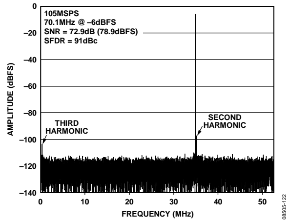
Figure 22. AD9255-105 Single-Tone FFT with f_{IN} = 70.1 MHz @ -6 dBFS with Dither Enabled
